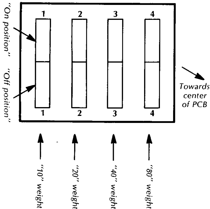
Figure 4-2 Detailed View of Bonus Credit Switch
