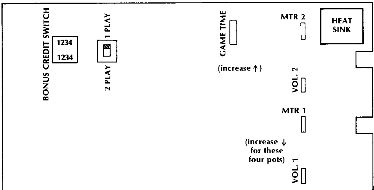
Figure 4-1 Approximate Locations of Owner/Operator Options on Crash 'N Score PCB
