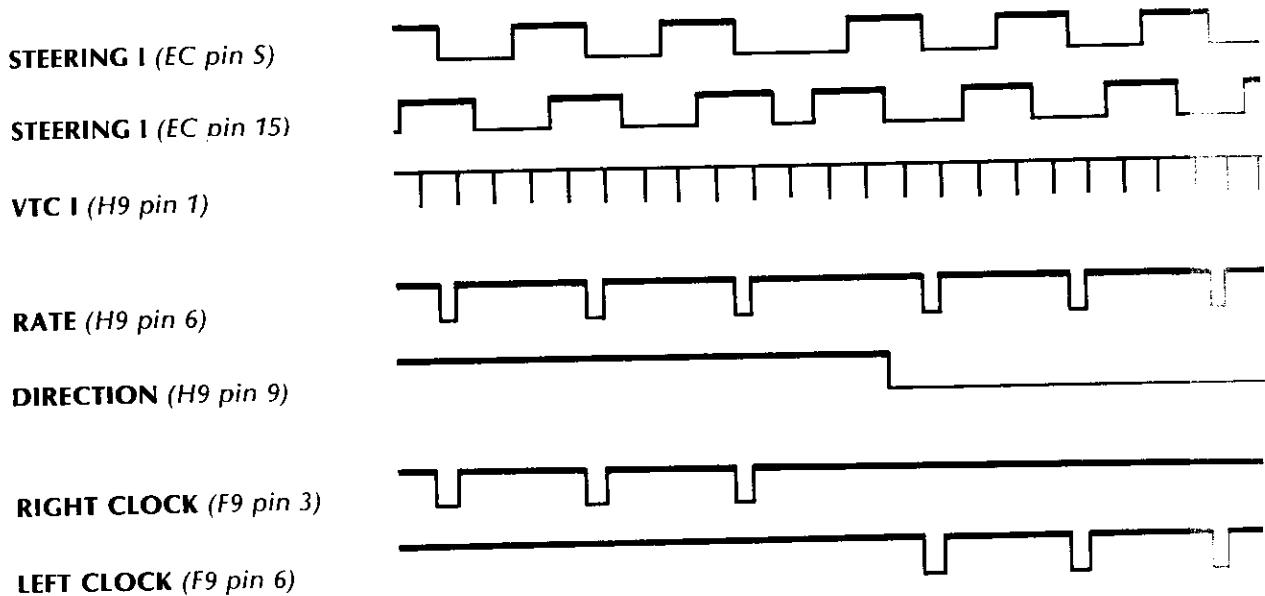
Figure 3-2 Sample Waveforms in Steering Decoder Circuit for Car I
