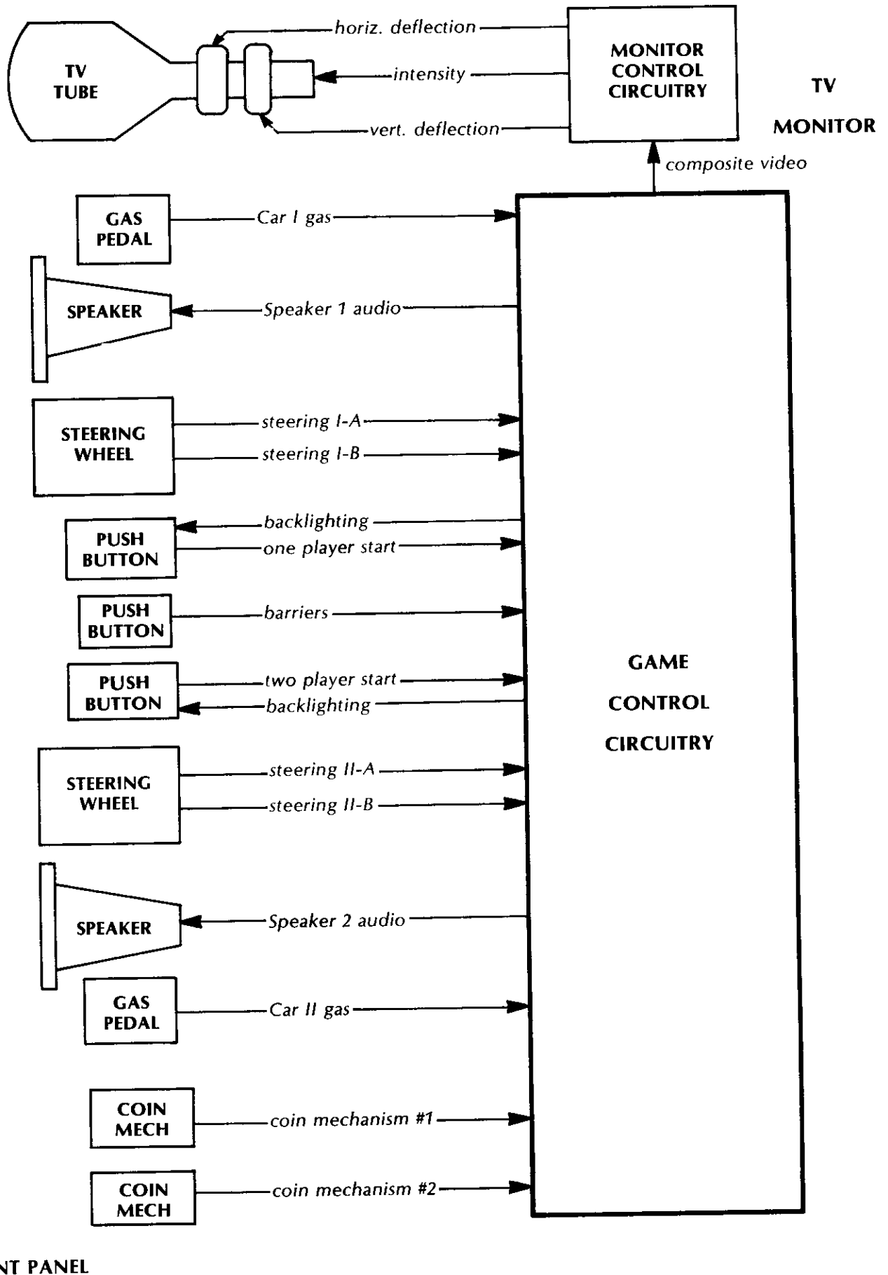
Figure 3-1 Block Diagram of Crash 'N Score Game
